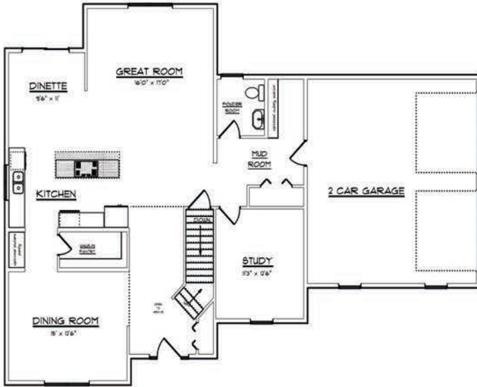
1 st Floor
